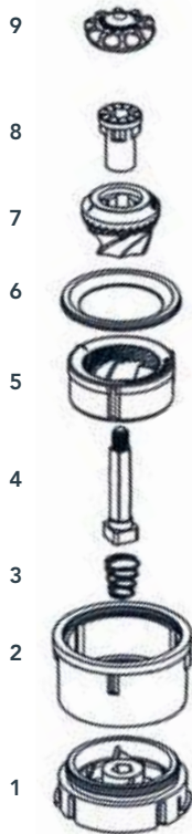
1. Base 2. Housing 3. Spring 4. Shaft 5. Crown 6. Bottom Ring 7. Cone 8. Cone holder 9. Adjusting wheel
